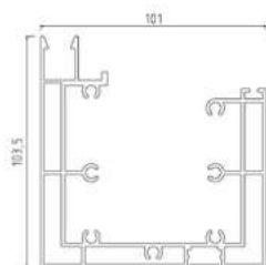
Gronda Laterale 3069 g/ml cod. NB0272
